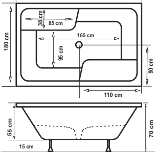
SW-5480 180 x 220 OPTİMUM ( YARIM OTURMALI ) 220 cm
