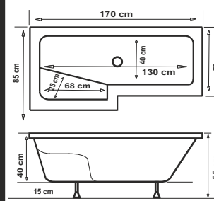
SW-5551 70 X 85 X 170 LOLA OTURMALI
